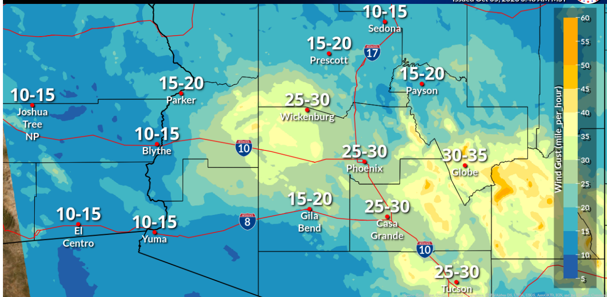
23-10-05_WindGust_Early_Saturday.png
